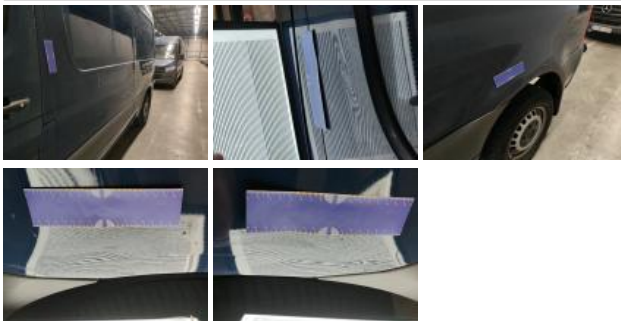
Wing trim RL, Scratch(es), Replace
